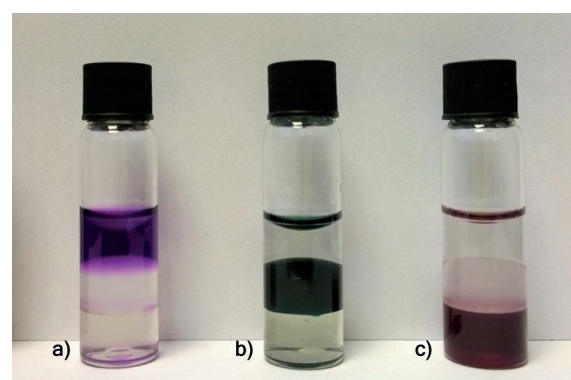
Figure 1. Equal volumes (0.5 mL) of water (top layer), [\text{P}_{6,6,6,14}][\text{NTf}_2] (middle layer), and [\text{emim}][\text{NTf}_2] (bottom layer) were added to each vial. A solid sample of cage 2 was added to the first vial, 3 to the second vial, and 4 to the third vial, respectively. Each vial was shaken vigorously for 10 seconds and allowed to settle before the photo was taken. a) Cage 2 is soluble only in water. b) Cage 3 is soluble only in [\text{P}_{6,6,6,14}][\text{NTf}_2] . c) Cage 4 is soluble only in [\text{emim}][\text{NTf}_2] .
